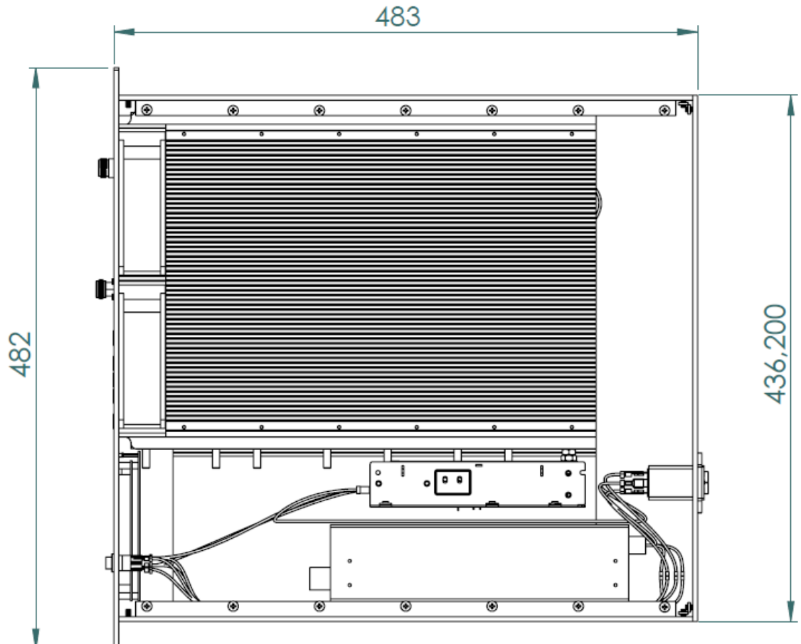
Figure 4 TOP VIEW (COVER REMOVED)
